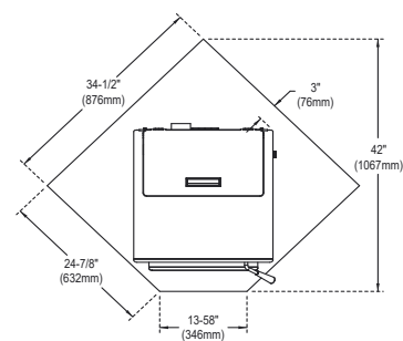
CORNER HEARTH PAD CLEARANCES
